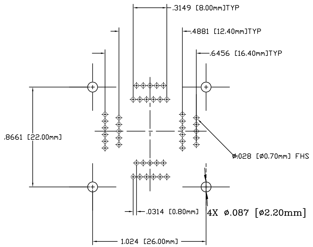
RECOMMENDED PCB LAYOUT AS SEEN FROM TOP OF SOCKET
