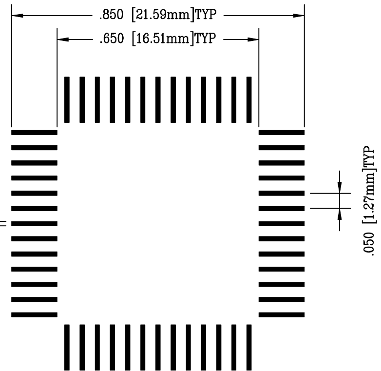
RECOMMENDED SMT LAYOUT
