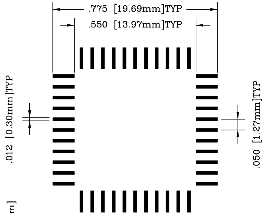
RECOMMENDED SMT LAYOUT
