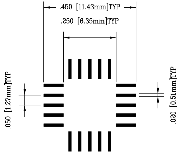
RECOMMENDED SMT LAYOUT
