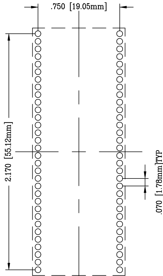
RECOMMENDED PCB LAYOUT AS SEEN FROM TOP OF SOCKET
