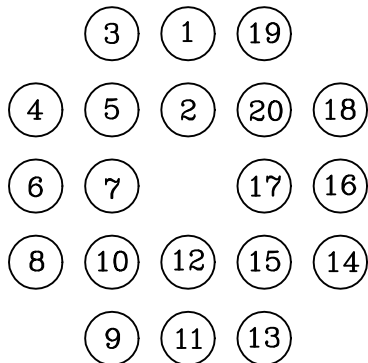
PIN MAP TOP VIEW
