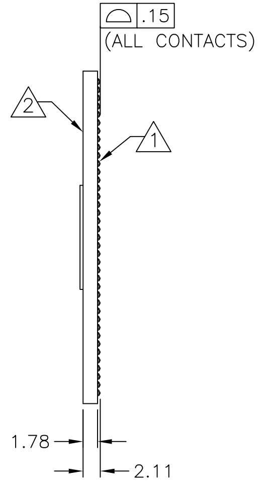
SIDE VIEW
