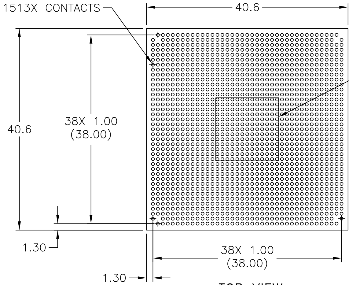
TOP VIEW
