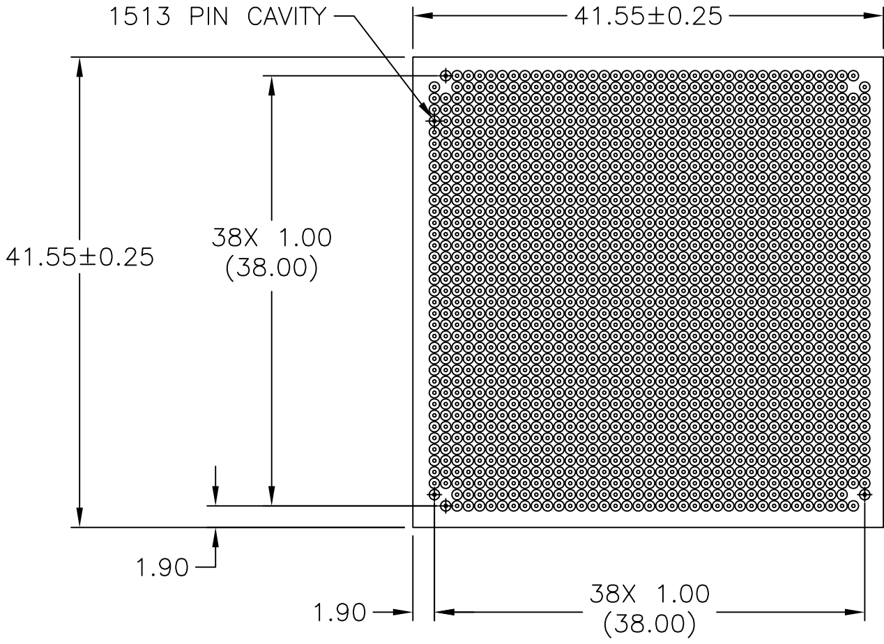
TOP VIEW
