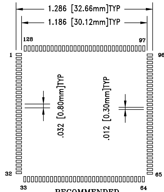
RECOMMENDED MINIMUM PAD LAYOUT
